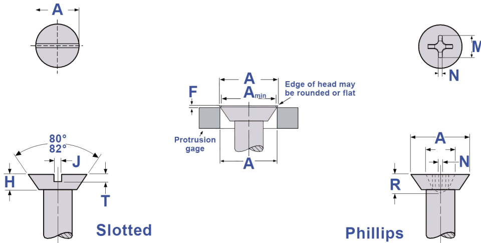
82 Degree Undercut Flat Head Machine Screws Slotted & Phillips Drive Dimensions
