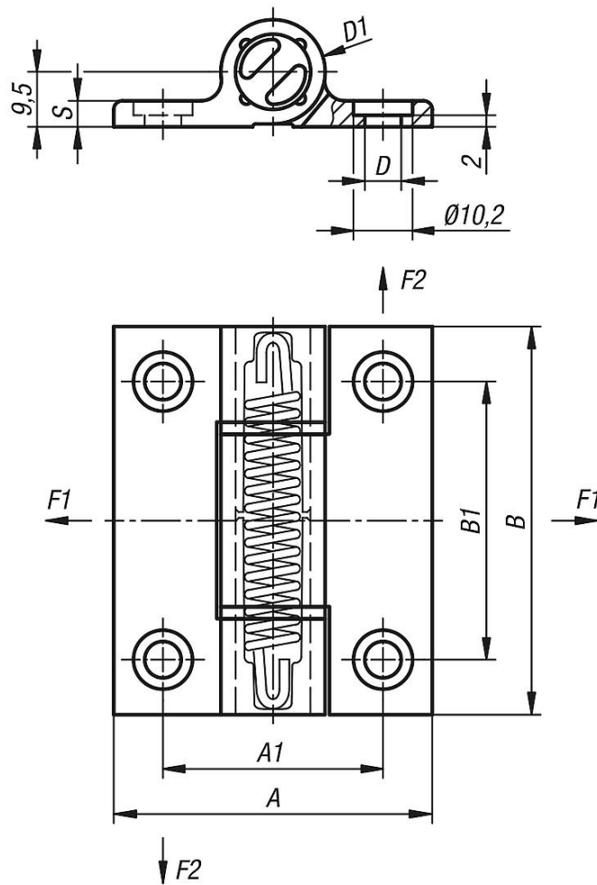
Hinges with opening spring
