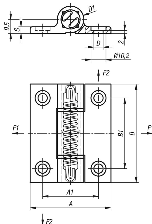
Hinges with opening spring
